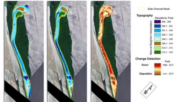
Figure 2. Changes in Buffalo Chute Morphology from 2007 to 2008.
